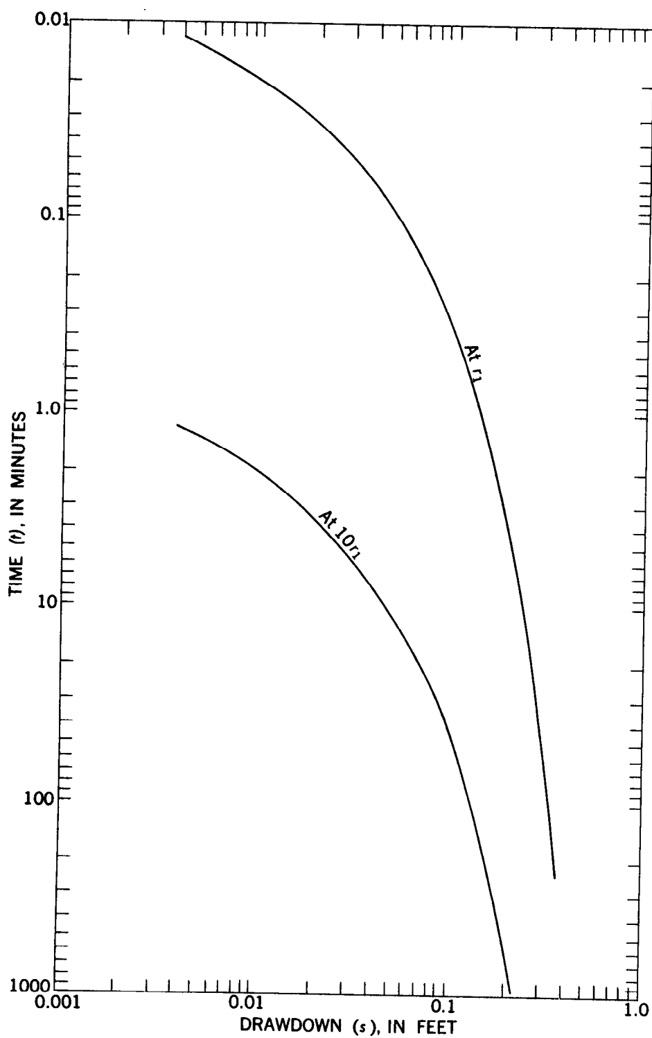
Figure 2.—Predicted response to pumping in observation wells.
