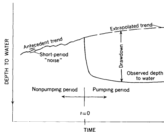
Figure 4.—Hydrograph for hypothetical observation well showing definition of drawdown.
